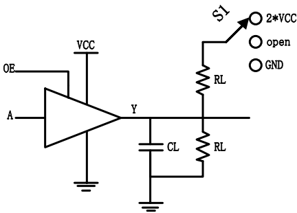
Figure5. Output enable/disable Time Test Circuit
