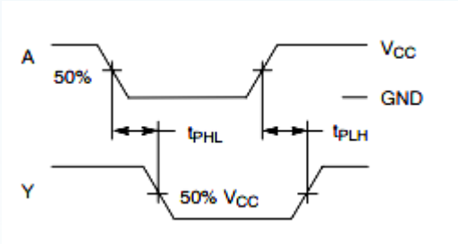
Figure3. Switch Waveform
