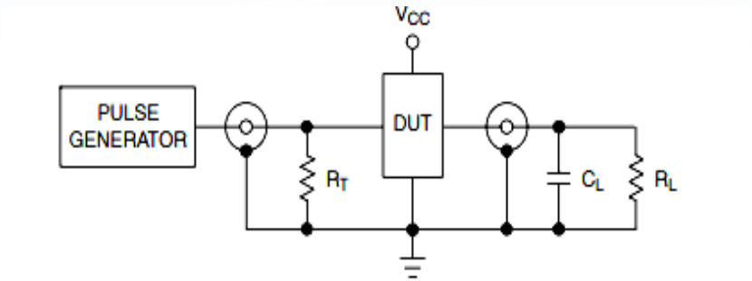
Figure4. Test Circuit
