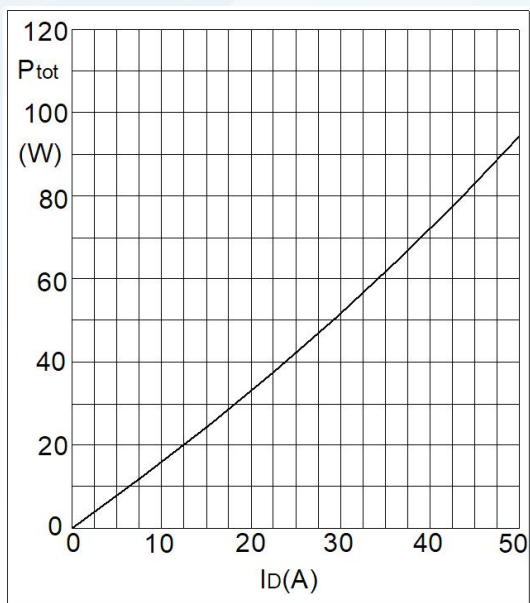
Fig1. Power Dissipation
