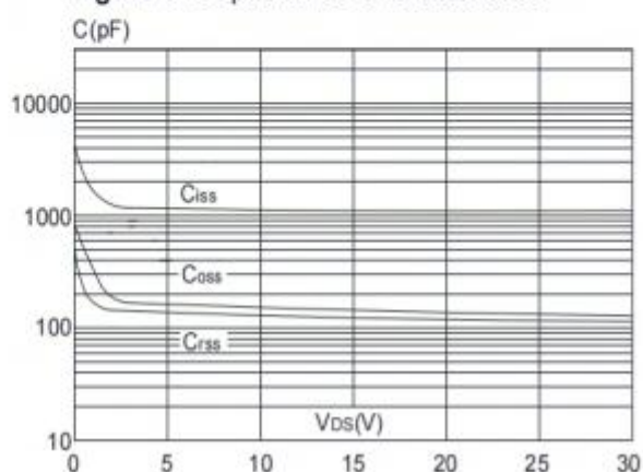
Figure 6: Capacitance Characteristics
