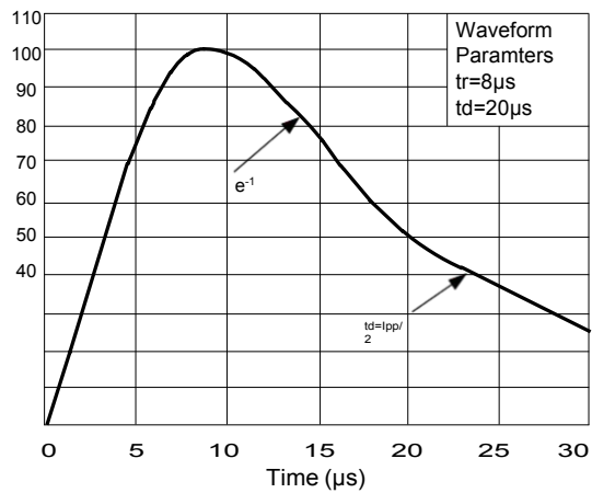
Figure3: Pulse Waveform
