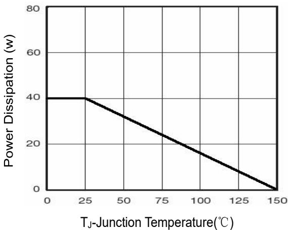
Figure 10 Power De-rating
