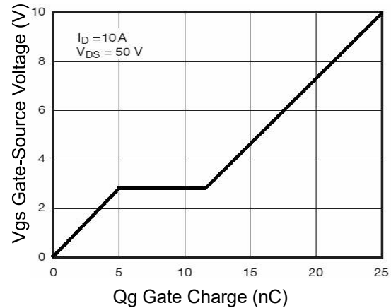
Figure 5 Gate Charge
