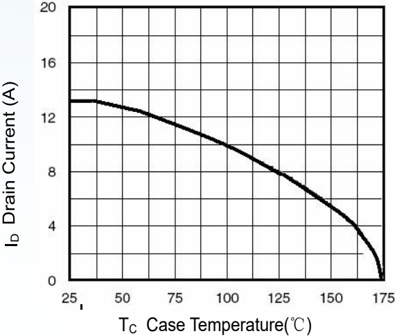
Figure 9 Drain Current vs Case Temperature
