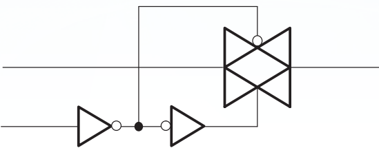
Figure 10. Logic Diagram (Positive Logic)
