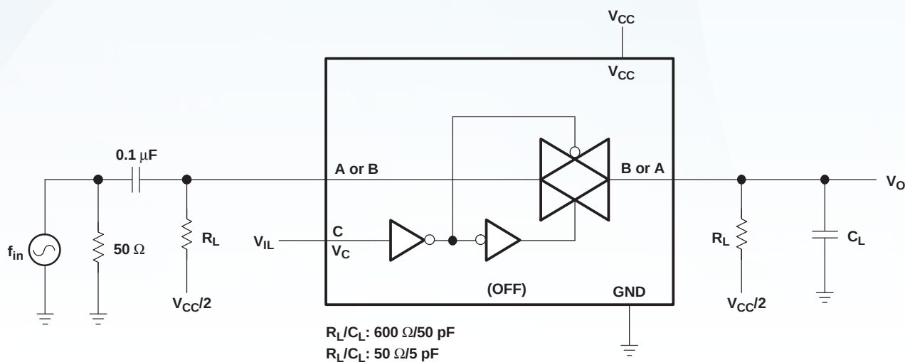
Figure 8. Feedthrough (Switch OFF)
