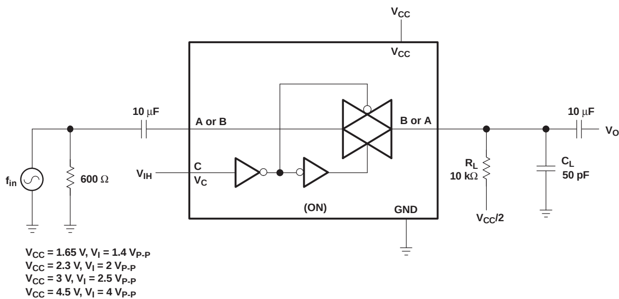
Figure 9. Sine-Wave Distortion
