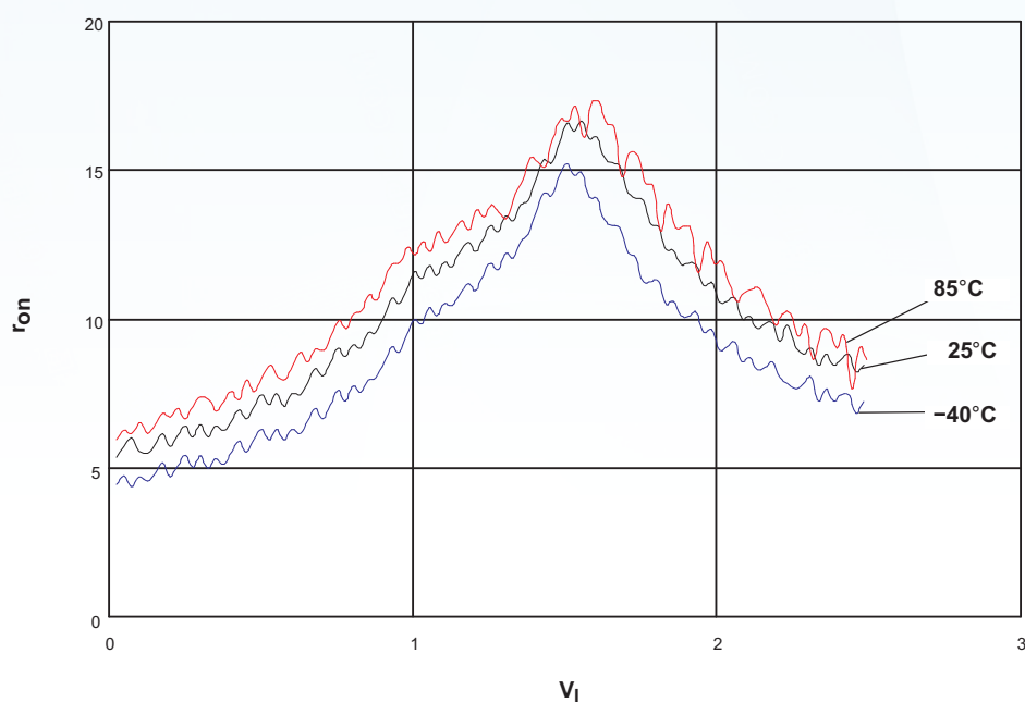
Figure 12. r_{on} vs V_I , V_{CC} = 2.5 V (SN74LVC1G66)
