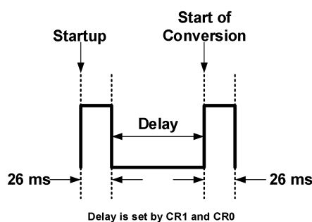
Figure 3. Schematic Diagram of Continuous Conversion
