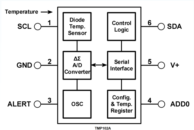
Figure 1. TMP102A Internal Schematic Diagram
