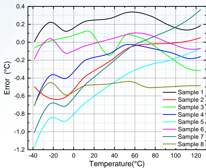
Figure 4. Temperature Error
