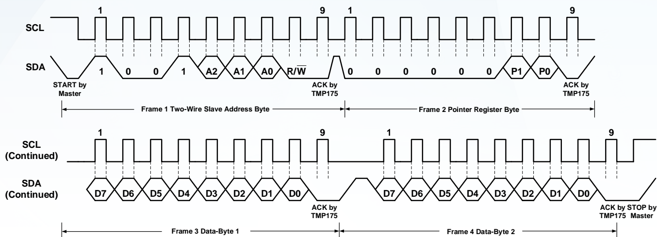
Figure 3. Two-wire Write Command Timing Diagram
