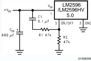
FIGURE 21. Delayed Startup
