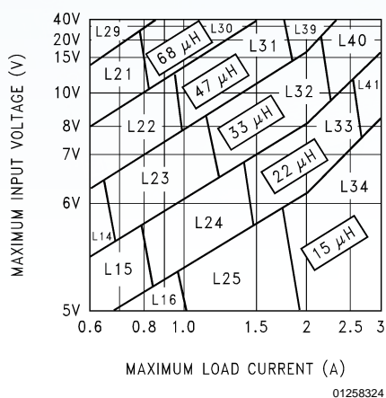
FIGURE 4. LM2596/LM2596HV-3.3
