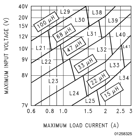
FIGURE 5. LM2596/LM2596HV-5.0
