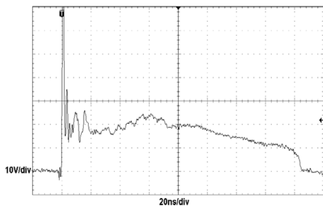
ESD clamping
