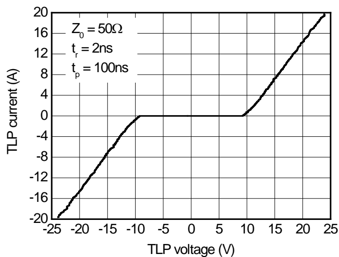
TLP Measurement
