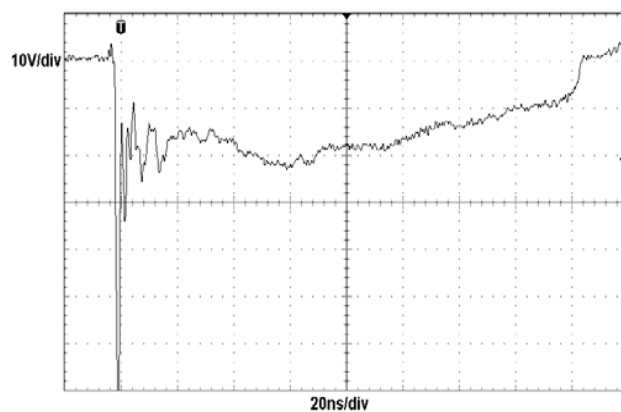
ESD clamping
