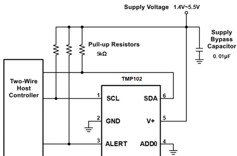
Figure 9. Typical Connections of the TMP102A
